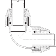
DİRSEK ELBOW
