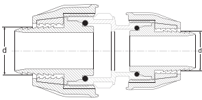
REDÜKSİYON MANŞON REDUCING COUPLING
